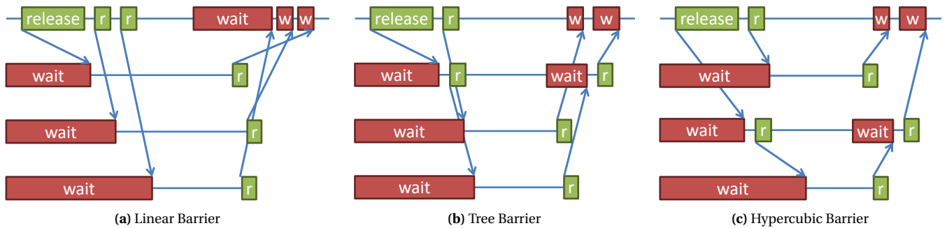
Figure 4: The blue arrows represent happens-before relations for fork/join barrier implementations in the Intel OpenMP Runtime.
